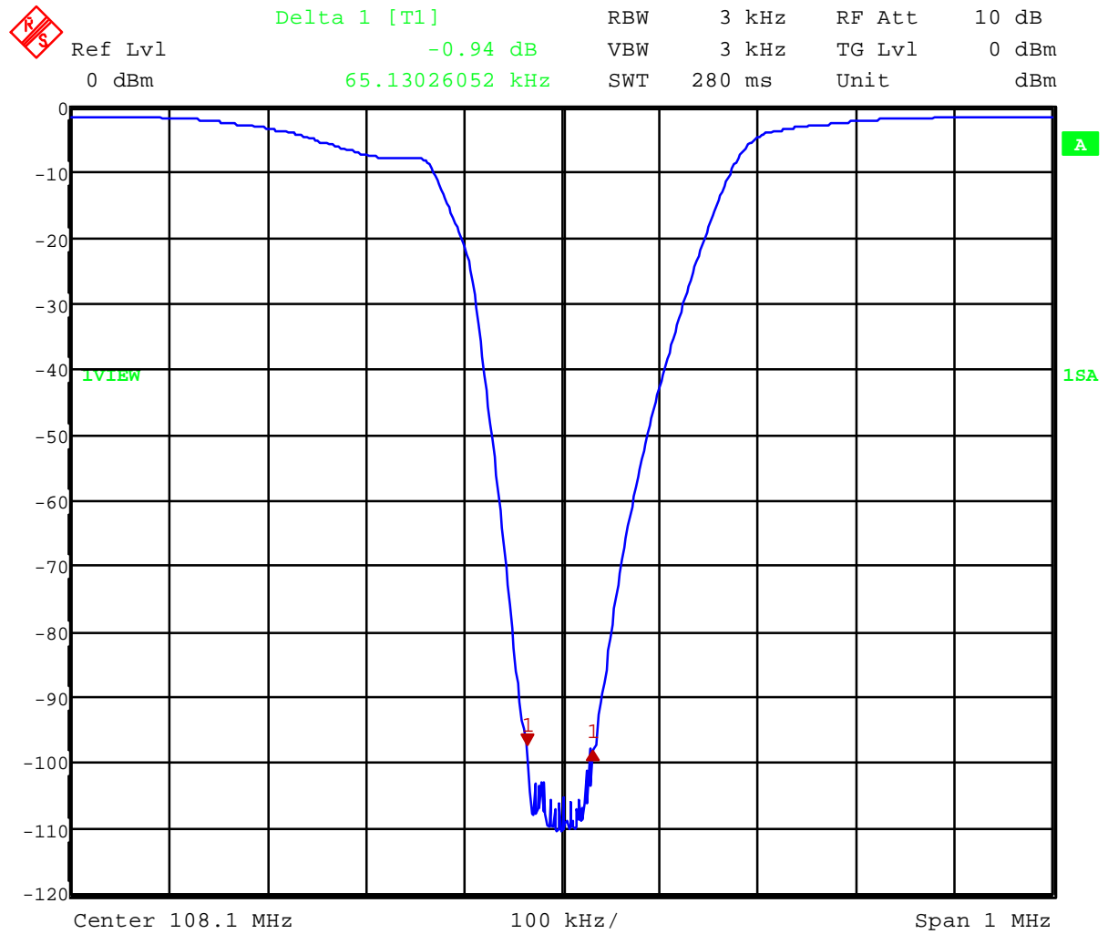
Fig. A2-3: Notch filter for the FM immunity measurements (series of nos. 22 to 24 in Annex 1)
