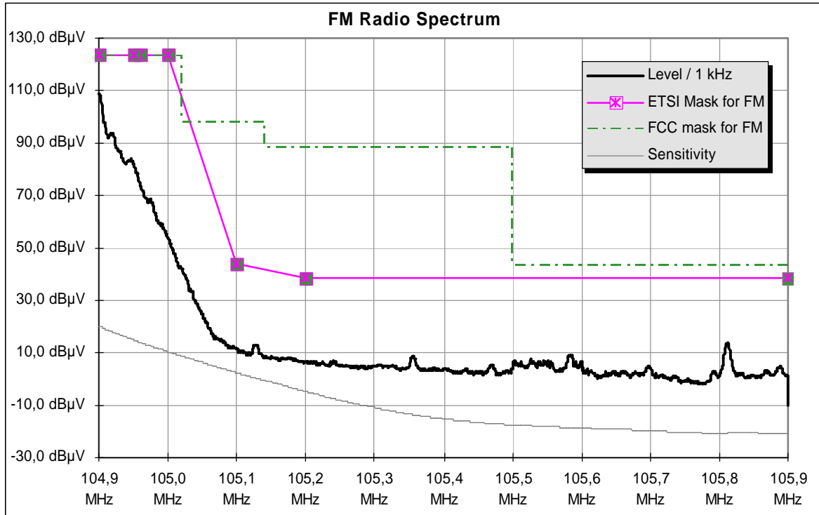
Fig. A2-1: High-dynamic spectrum recording of the upper sideband of the standard FM unwanted signal from the Itelco transmitter, modulated according to ITU-R IS.1140.
