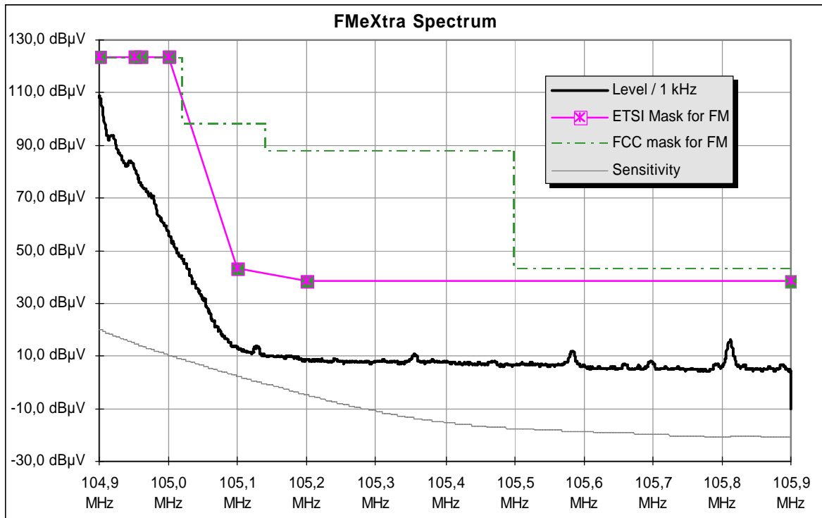
Fig. A2-2: High-dynamic spectrum recording of the upper sideband of the FMExtra unwanted signal from the ITELCO transmitter, modulated according to ITU-R IS.1140.
