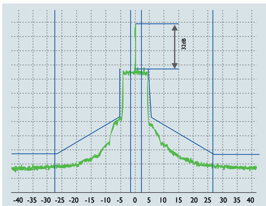
Figure 9.2.8: DRM spectrum with additional carrier
