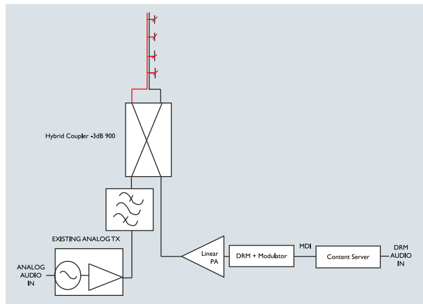
Figure 9.3.3.2b: DRM+ Combined Mode – split feed Antenna coupling
