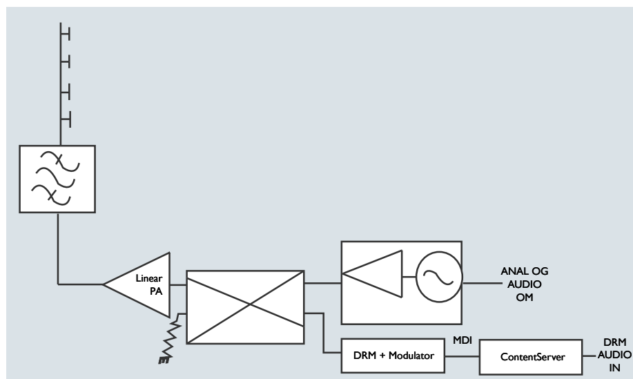
Figure 9.3.4: DRM+ and FM combining at low signal level
