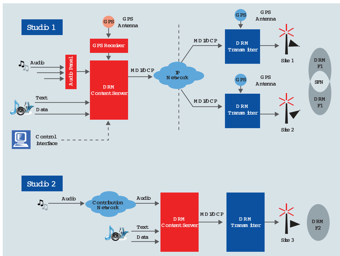
Figure 9.1.1b: Typical DRM local/regional/national broadcast network topology
