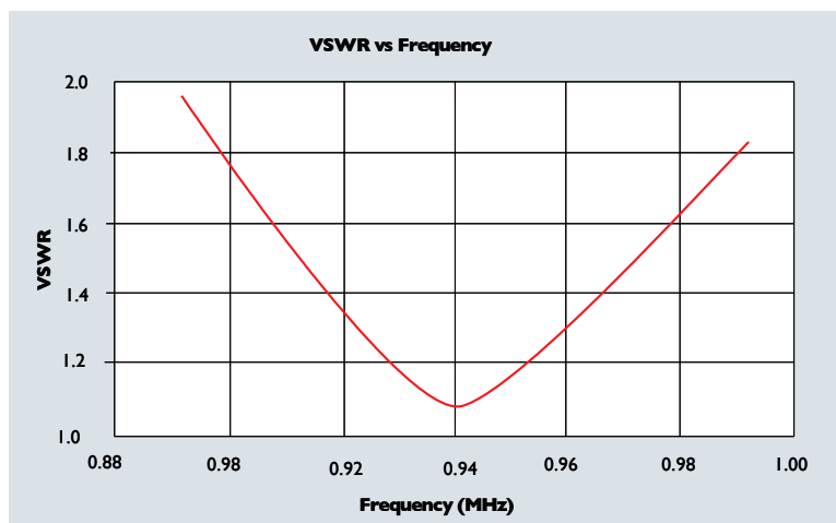
Figure 9.7.1: Typical VSWR of an MF \lambda/4 Antenna Power
