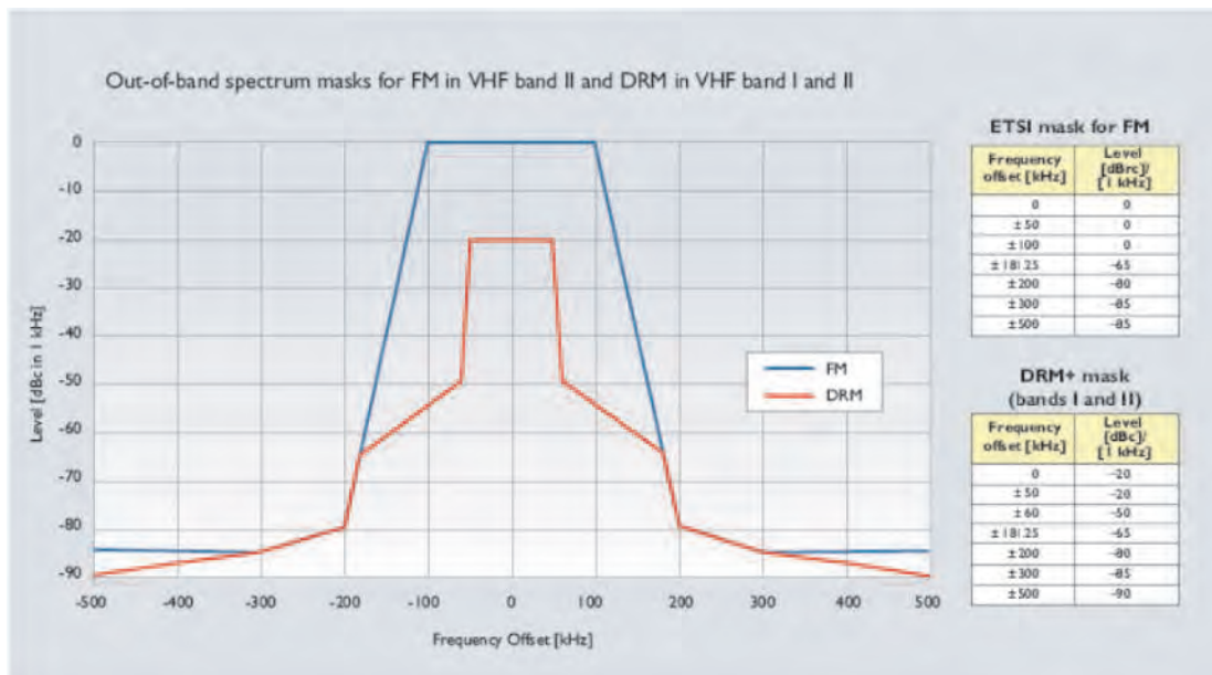
Figure 9.4.1a Spectrum mask for DRM+ and FM broadcast
