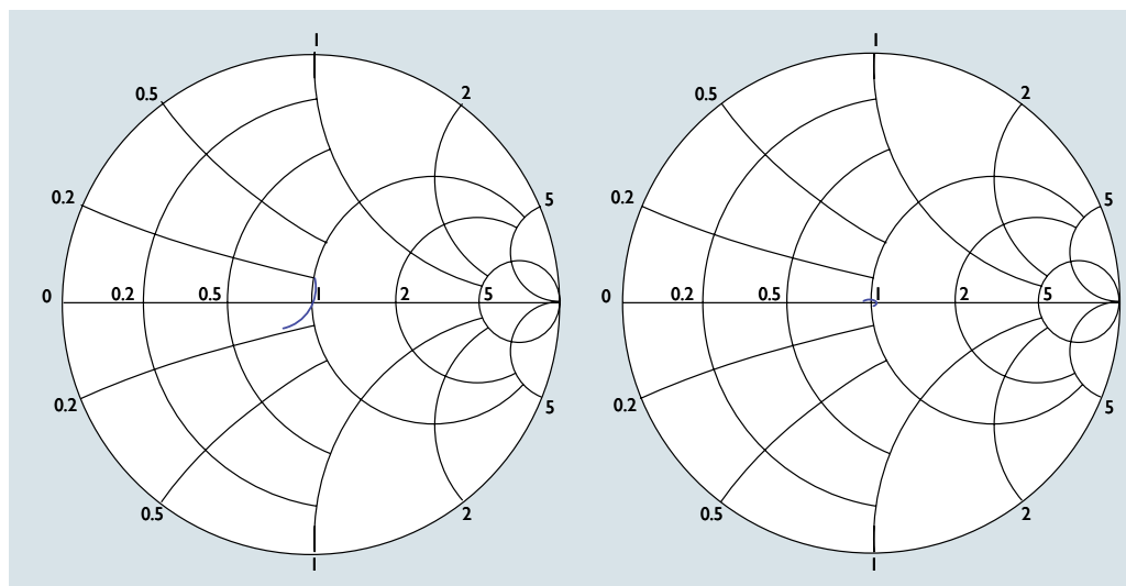
Figure 9.7.2b: LF Antenna Smith Chart: left – antenna only; right – including ATU
