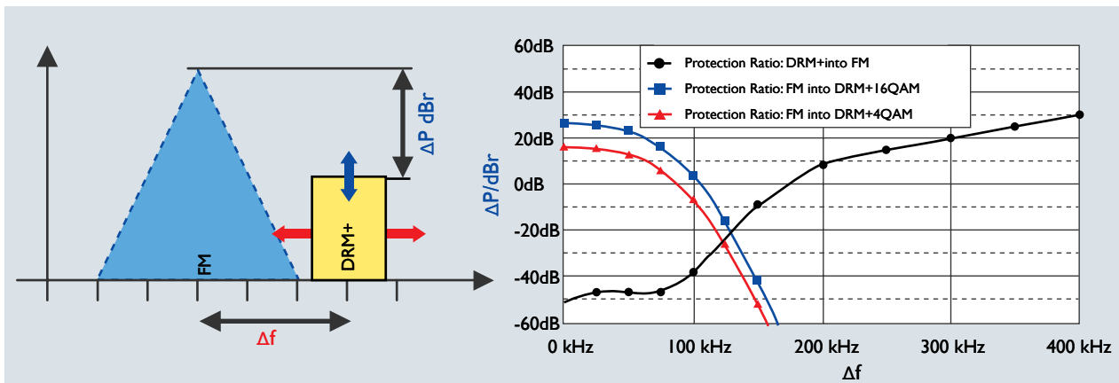
Figure 9.4.1b DRM+ combined mode power setup and protection levels
