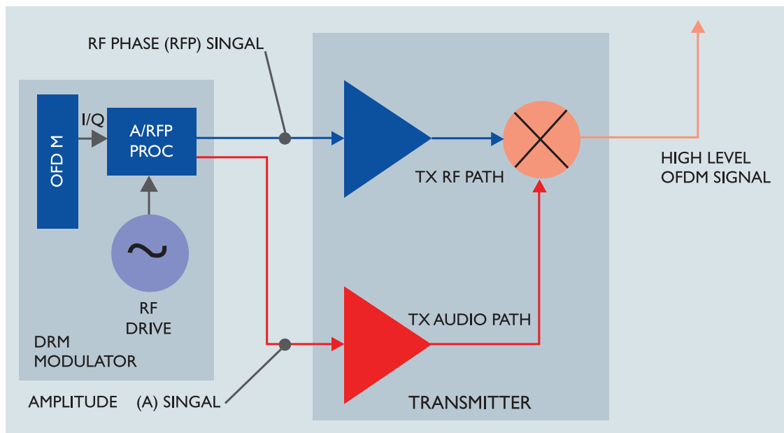
Figure 9.2.5: DRM Transmitter with A/RFP topology
